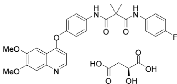
Figure 1: Chemical structure of cabozantinib (S)-malate
