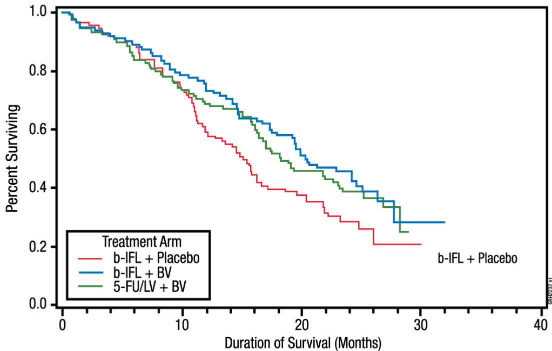
Figure 3: Plot of Kaplan Meier Estimates for survival in study AVF2107g: Patients enrolled in Arm 3 and concurrently enrolled patients in Arms 1 and 2
