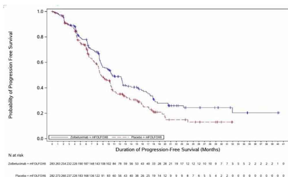
Figure 1. Kaplan Meier plot of progression free survival, SPOTLIGHT (primary analysis)
